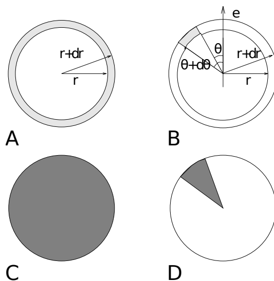
Fig. 5.52: Definition of slices in gmx rdf (page 245): A. g_{AB}(r) . B. g_{AB}(r, \theta) . The slices are colored gray. C. Normalization \langle \rho_B \rangle_{local} . D. Normalization \langle \rho_B \rangle_{local, \theta} . Normalization volumes are colored gray.
